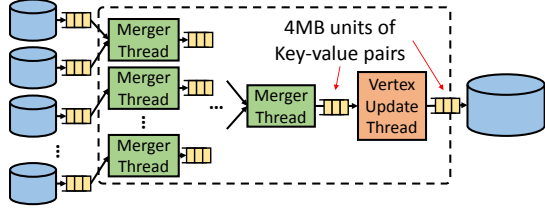
Figure 11: A multithreaded software implementation of sort-reduce
