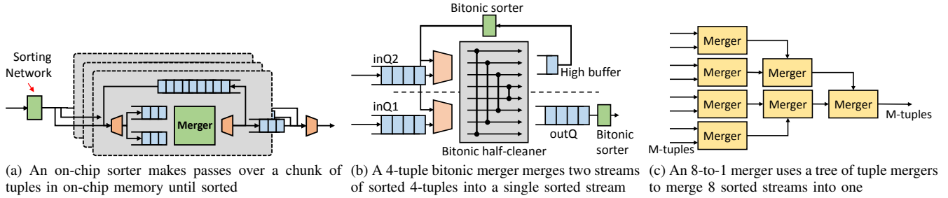
Figure 9: Accelerators components involved in sort-reduce
