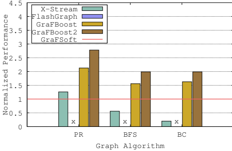
(a) Performance of the algorithms on the Kronecker 32 graph, on a machine with 128 GB of memory, normalized to the performance of software GraFBoost ( Higher is faster )
