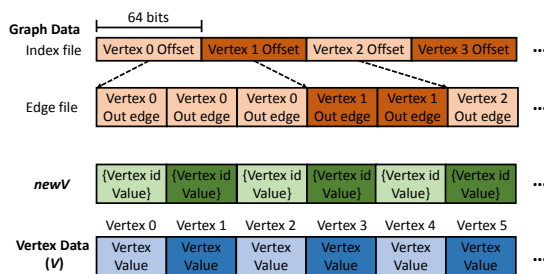
Figure 6: Compressed column representation of graph structure
