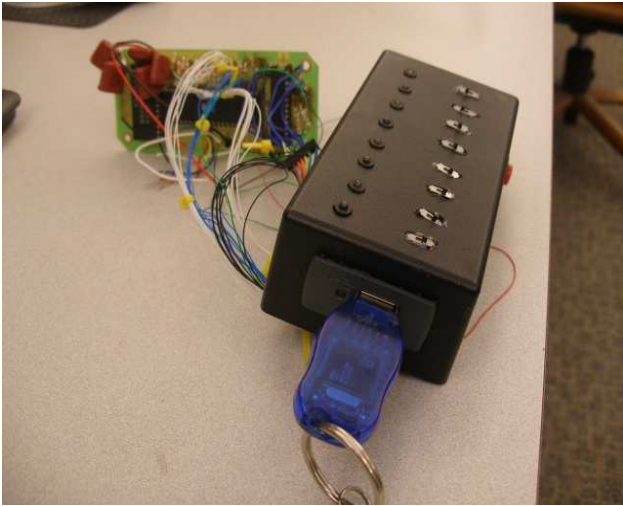
Figure 7: Virtual microcontroller implementations- Implementation # 1: in a black-box, with internal AVR-microcontroller-based circuitry exposed.
