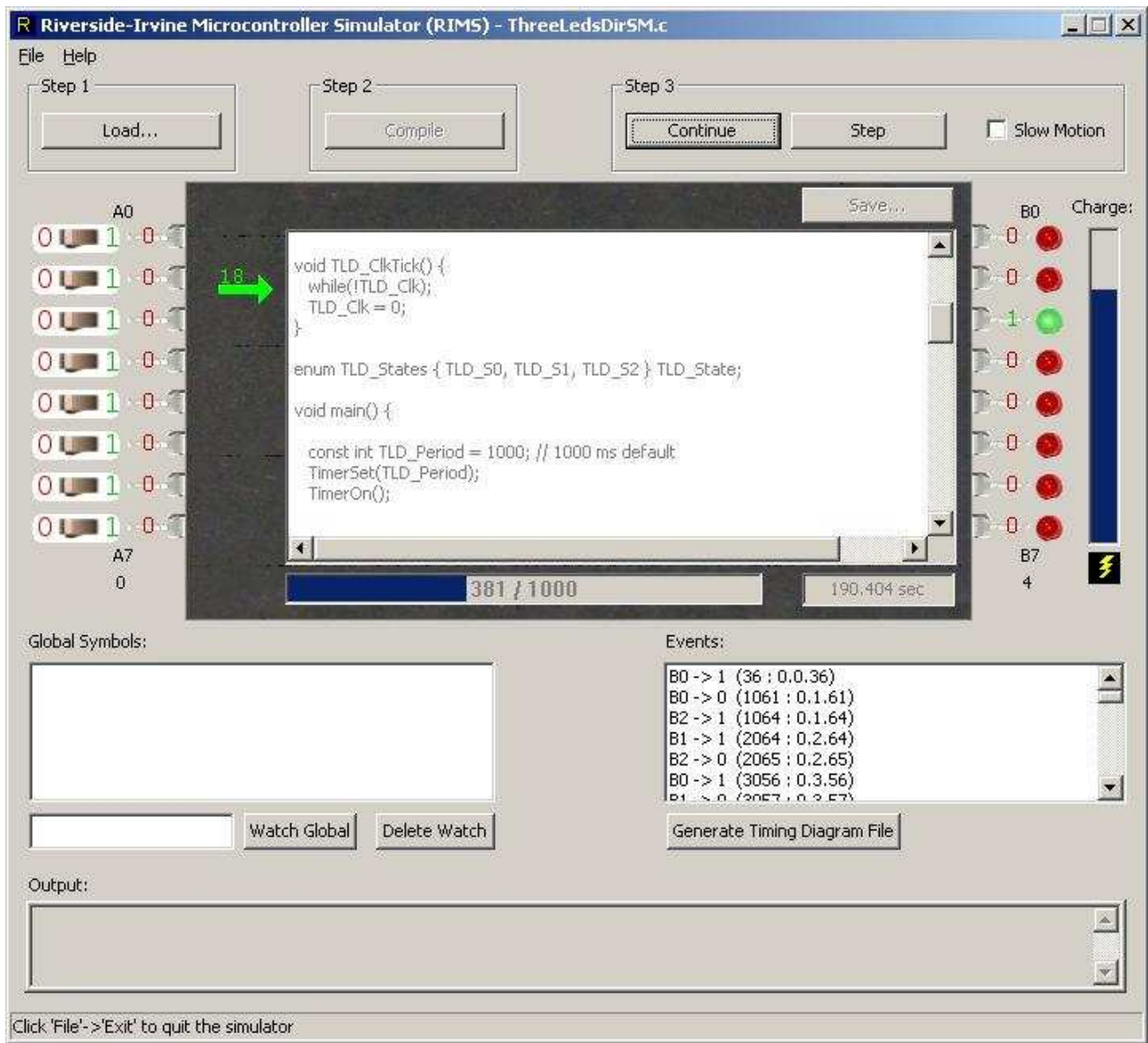
Figure 6: Virtual microcontroller simulator prototype. The simulator supports standard debugger and register views, as well as a high level view of the virtual microcontroller and connected peripherals. The simulator also reports power usage, indicated on the right by a battery indicator.
