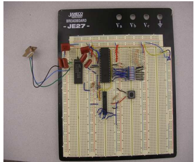
Figure 8: Implementation # 2: on an AVR microcontroller breadboard, with input/output wires that can be connected to other circuits
