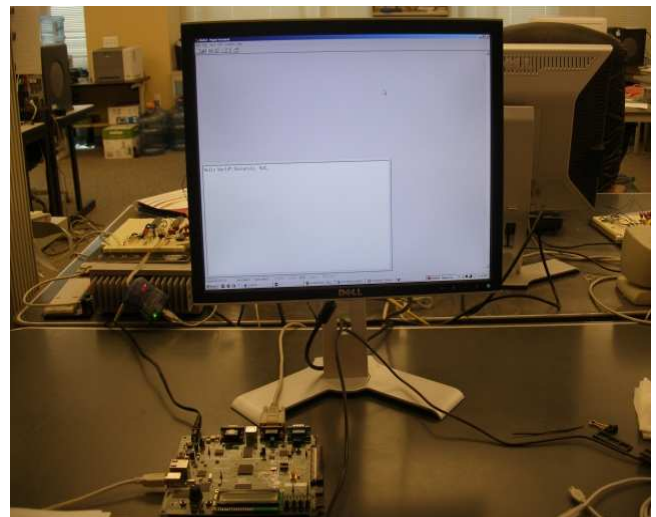
Figure 9: Implementation # 3: on a Xilinx Spartan 3E FPGA using a serial connection to a PC to output to a serial terminal.
