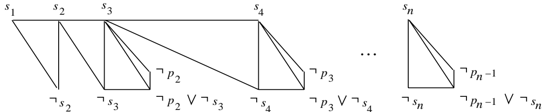
Figure 4: Interaction graph for Example 6.2
