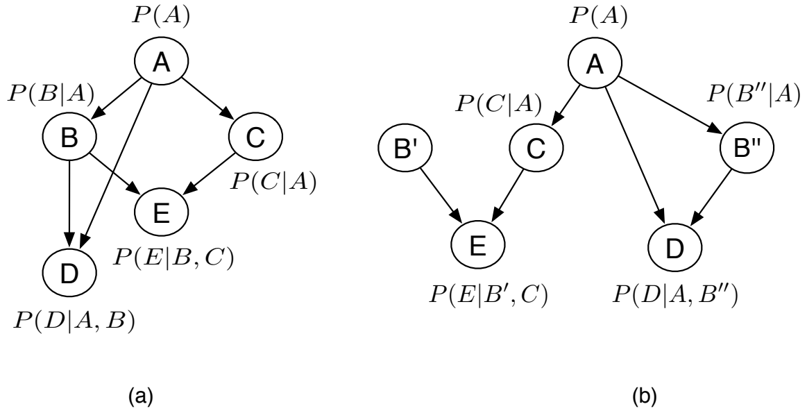
Figure 1.3: (a) The original Bayesian network, (b) The network with duplicated variable B and P(B|A) . The question of how to best distribute the functions between mini-buckets is not trivial and is usually solved heuristically. More information can be found in [81].
