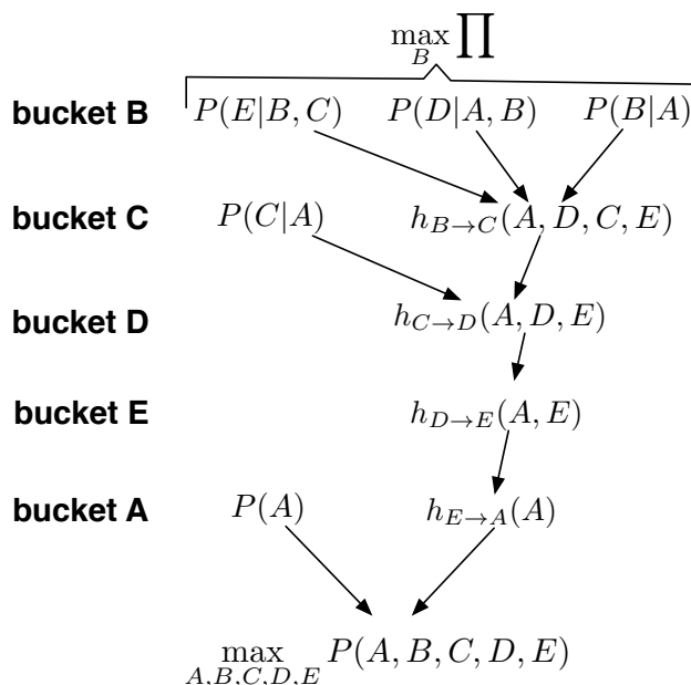
Figure 1.2: A trace of bucket elimination algorithm
