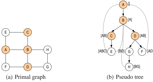
Figure 1: A simple graphical model.
