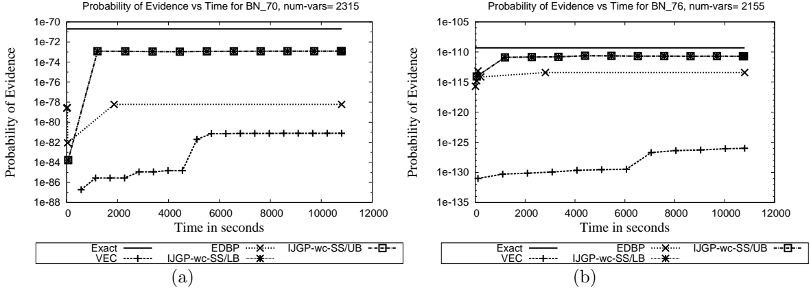
Figure 8: Convergence of probability of evidence as a function of time for two sample Linkage instances. IJGP-wc-IS is not plotted in the figures because it fails on all the instances.
