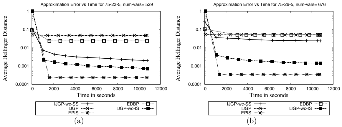
Figure 13: Time versus Hellinger distance \Delta between the exact and approximate marginals for IJGP-wc-IS, IJGP-wc-SS, IJGP, EPIS and EDBP for two sample Grid instances with deterministic ratio=75% .
