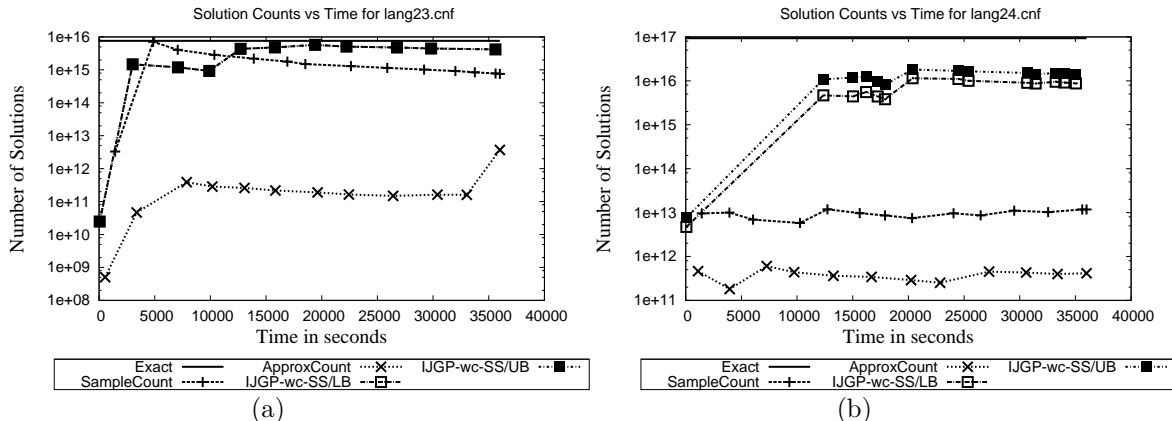
Figure 6: Time versus solution counts for two sample Langford instances. IJGP-wc-IS and Relsat are not plotted in the figures because they fail on the given instances.
