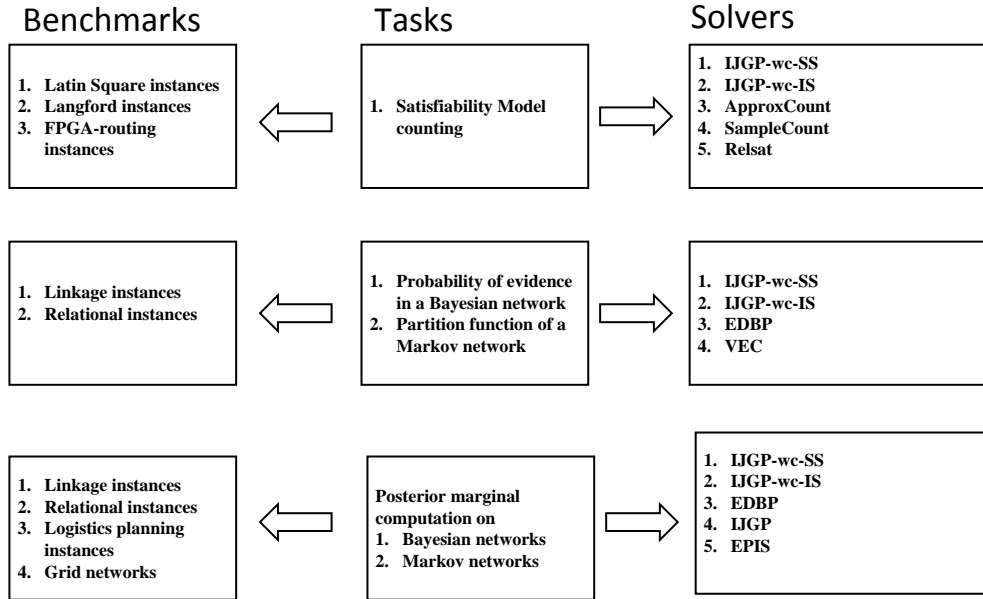
Figure 4: Chart showing the scope of our experimental study
