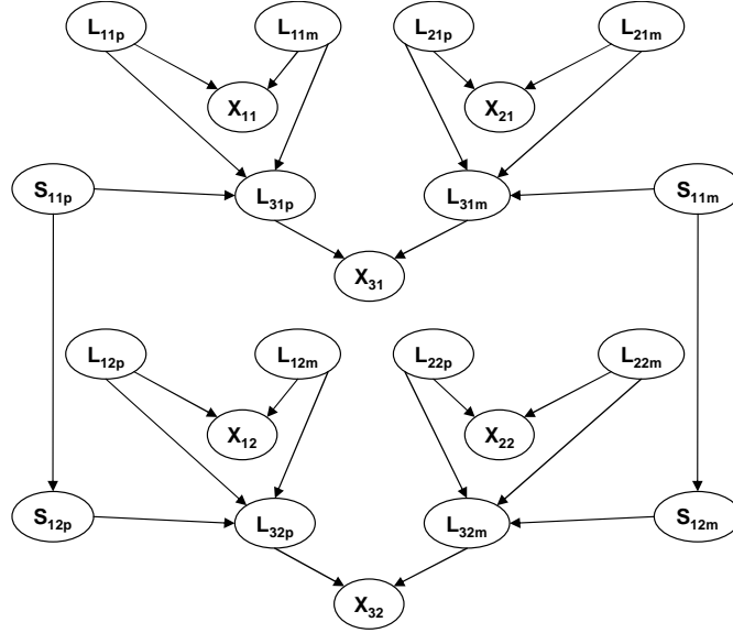
Figure 7: A fragment of a Bayesian network used in genetic linkage analysis.
