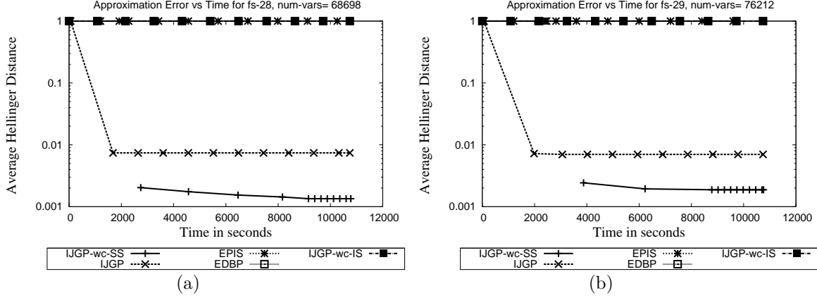
Figure 10: Time versus Hellinger distance \Delta between the exact and approximate marginals for IJGP-wc-IS, IJGP-wc-SS, IJGP, EPIS and EDBP for two sample Friends and Smokers networks.
