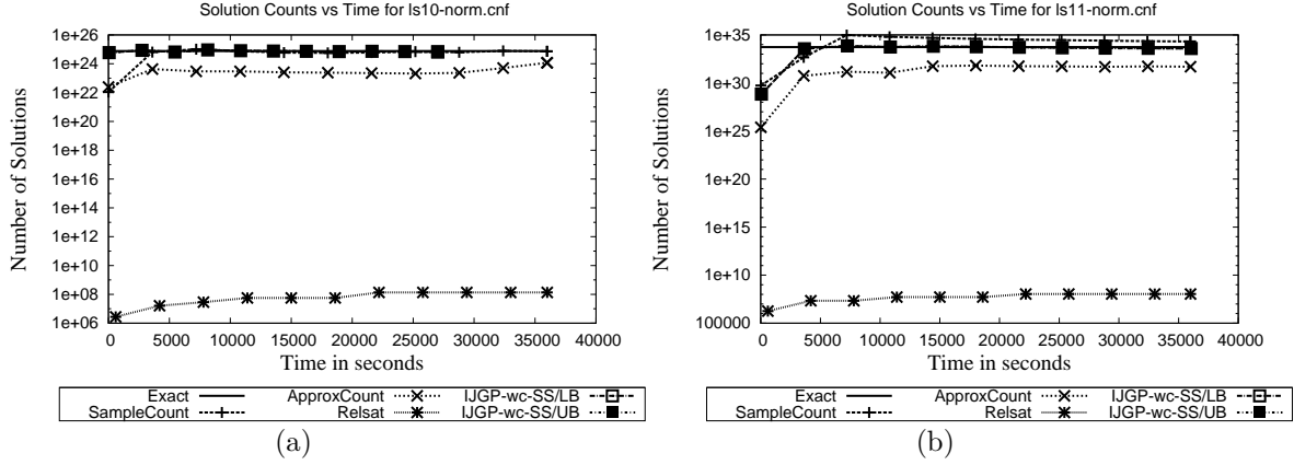
Figure 5: Time versus solution counts for two sample Latin square instances. IJGP-wc-IS is not plotted in the figures because it fails on all the instances.
