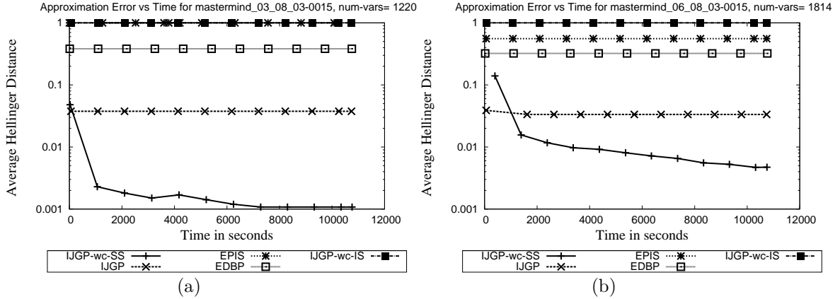
Figure 11: Time versus Hellinger distance \Delta between the exact and approximate marginals for IJGP-wc-IS, IJGP-wc-SS, IJGP, EPIS and EDBP for two sample Mastermind networks.
