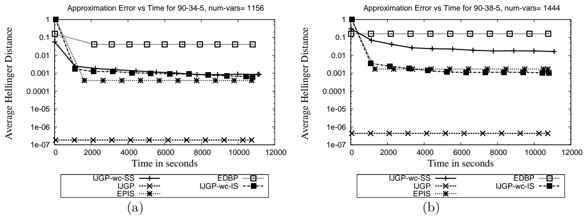
Figure 14: Time versus Hellinger distance \Delta between the exact and approximate marginals for IJGP-wc-IS, IJGP-wc-SS, IJGP, EPIS and EDBP for two sample Grid instances with deterministic ratio=90% .
