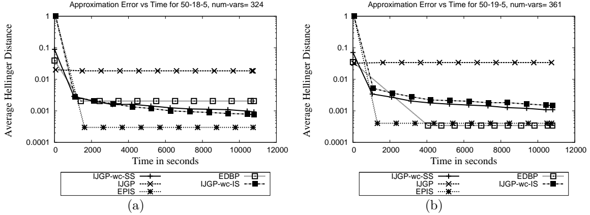
Figure 12: Time versus Hellinger distance \Delta between the exact and approximate marginals for IJGP-wc-IS, IJGP-wc-SS, IJGP, EPIS and EDBP for two sample Grid instances with deterministic ratio=50% .
