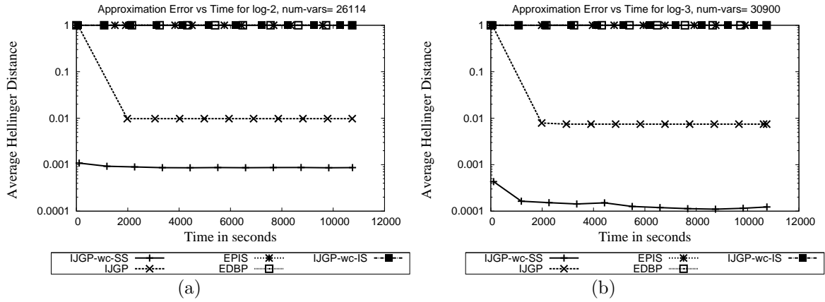
Figure 15: Time versus Hellinger distance \Delta between the exact and approximate marginals for IJGP-wc-IS, IJGP-wc-SS, IJGP, EPIS and EDBP for two sample Logistics planning instances .
