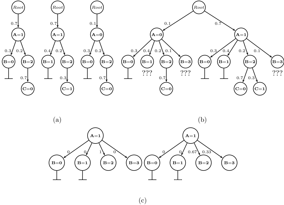
Figure 3: (a) Three DFS-traces (b) Combined information from the three DFS-traces given in (a) and (c) Two possible approximations of I(B|A = 1)
