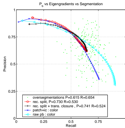
Figure 9: This figure shows that in passing from gradients of eigenvectors to segmentations, we are able to maintain high precision in identifying true boundaries. The cloud of points correspond to the initial oversegmentations for the set of images. The red ( \circ ) curve shows the results of recursively splitting the graph corresponding to this oversegmentation. The black curve ( + ) shows the results of the same procedure using weights which have been extended by setting undefined edges between a pair of superpixels to be the average of the defined weights.
