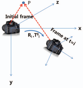
Figure 3. Basic kinematics: To estimate the blur kernel, 3D homography is used to reflect the 6-DoF camera motion to the pixel ( P in the figure).
