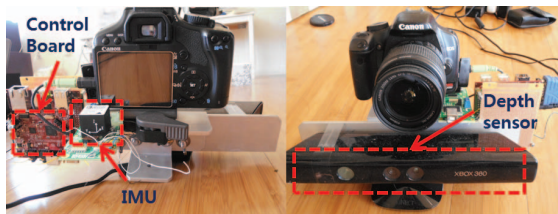
Figure 1. The system picture: The system is composed of DSLR camera (Canon EOS450d with 18-35mm lens), IMU (Analog devices, ADIS16350), Depth sensor (Microsoft Kinect), and Control board (Beagleboard-xm)
