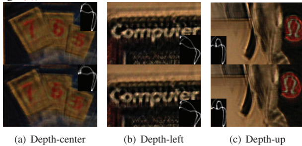
Figure 8. Blur kernel with the depth map and without the depth map: The first row of the images are the latent image from the blur kernel estimated using IMU data and the depth map. The second row are the latent image from the IMU data and constant depth for all three image patches. The estimated blur kernels are shown in each image.
